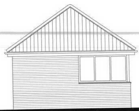
Front Elevation 1:100 as proposed
