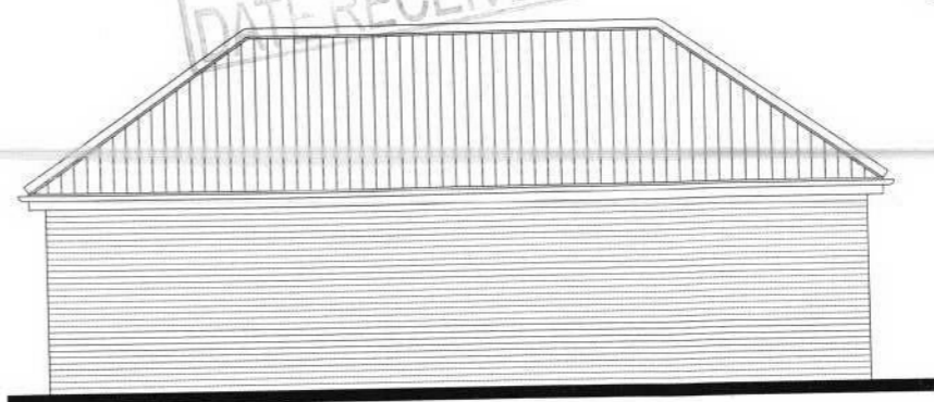
Side Elevation 1:100 as proposed
