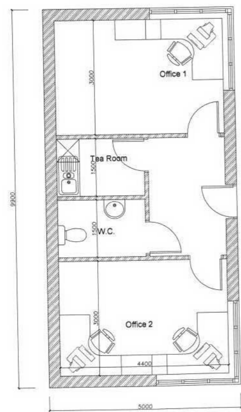
Ground Floor Plan - 1:100 as proposed
