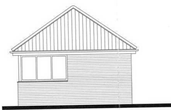
Rear Elevation 1:100 as proposed
